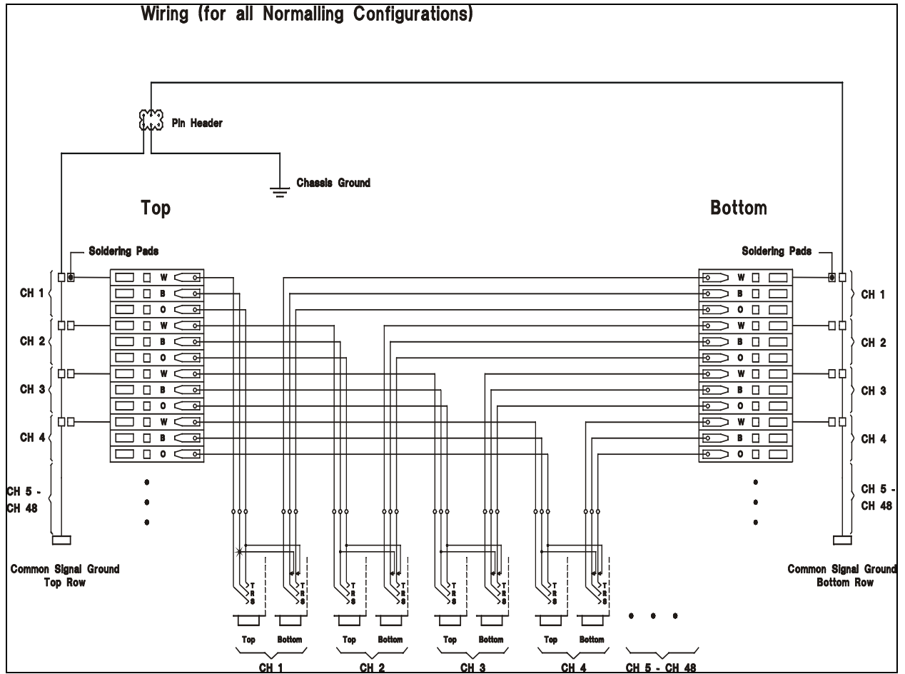
Wiring diagram
