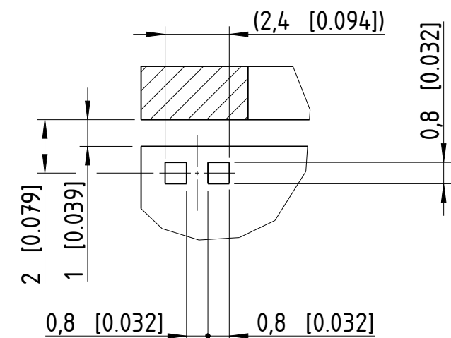
Detail X 5:1
